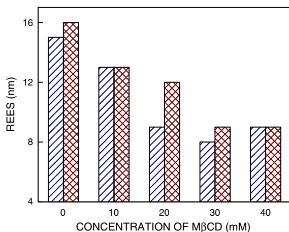
Fig. 4. Effect of cholesterol depletion on the magnitude of REES of NR12S in native hippocampal membranes, and in liposomes of lipid extract from native membranes. REES of NR12S, corresponding to total shift in emission maximum when the excitation wavelength was changed from 510 to 570 nm, in native membranes (hatched bar) and in liposomes of lipid extract (crisscrossed bar) from native membranes are shown with increasing cholesterol depletion using 10–40 mM M \beta CD. All other conditions are as in Fig. 2. See Materials and methods for other details.
