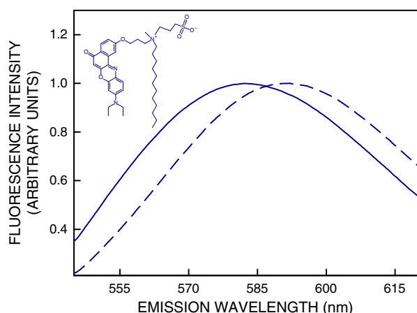
Fig. 2. Representative fluorescence emission spectra of NR12S in native (—) and cholesterol-depleted (---) hippocampal membranes. The concentration of MβCD used was 40 mM. The spectra are intensity-normalized at the respective emission maxima. Measurements were carried out at room temperature ( \sim 23 °C). The excitation wavelength used was 510 nm. The ratio of NR12S to total lipid was 1:100 (mol/mol). The chemical structure of NR12S is also shown. See Materials and methods for other details.
