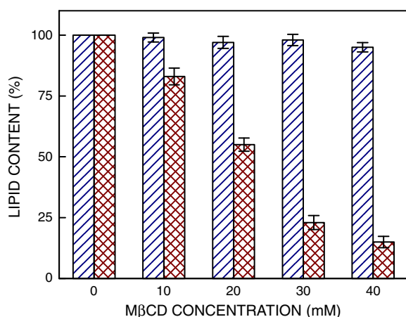
Fig. 1. Effect of MβCD on the lipid content of hippocampal membranes. The figure shows phospholipid (hatched bar) and cholesterol (crisscrossed bar) contents in hippocampal membranes treated with increasing concentrations of MβCD. Values are expressed as percentages of phospholipid and cholesterol contents in native hippocampal membranes without MβCD treatment. Data represent means \pm S.E. of at least four independent measurements. See Materials and methods for other details.
