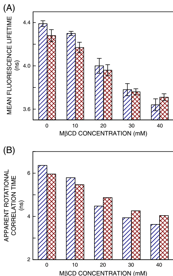
Fig. 8. (A) Effect of cholesterol depletion on mean fluorescence lifetime of NR12S in native hippocampal membranes (hatched bar) and in liposomes of lipid extract from native membranes (crisscrossed bar). Mean fluorescence lifetimes were calculated using Eq. (3). The excitation wavelength used was 490 nm and emission was monitored at 585 nm. Data shown are means \pm S.E. of at least three independent measurements. All other conditions are as in Fig. 2. See Materials and methods for other details. (B) Apparent rotational correlation times of NR12S in native hippocampal membranes (hatched bar) and in liposomes of lipid extract from native membranes (crisscrossed bar) with increasing cholesterol depletion. Apparent rotational correlation times were calculated from fluorescence anisotropy values of NR12S from Fig. 7 and mean fluorescence lifetimes from panel (A) using Eq. (4). See text for other details.
